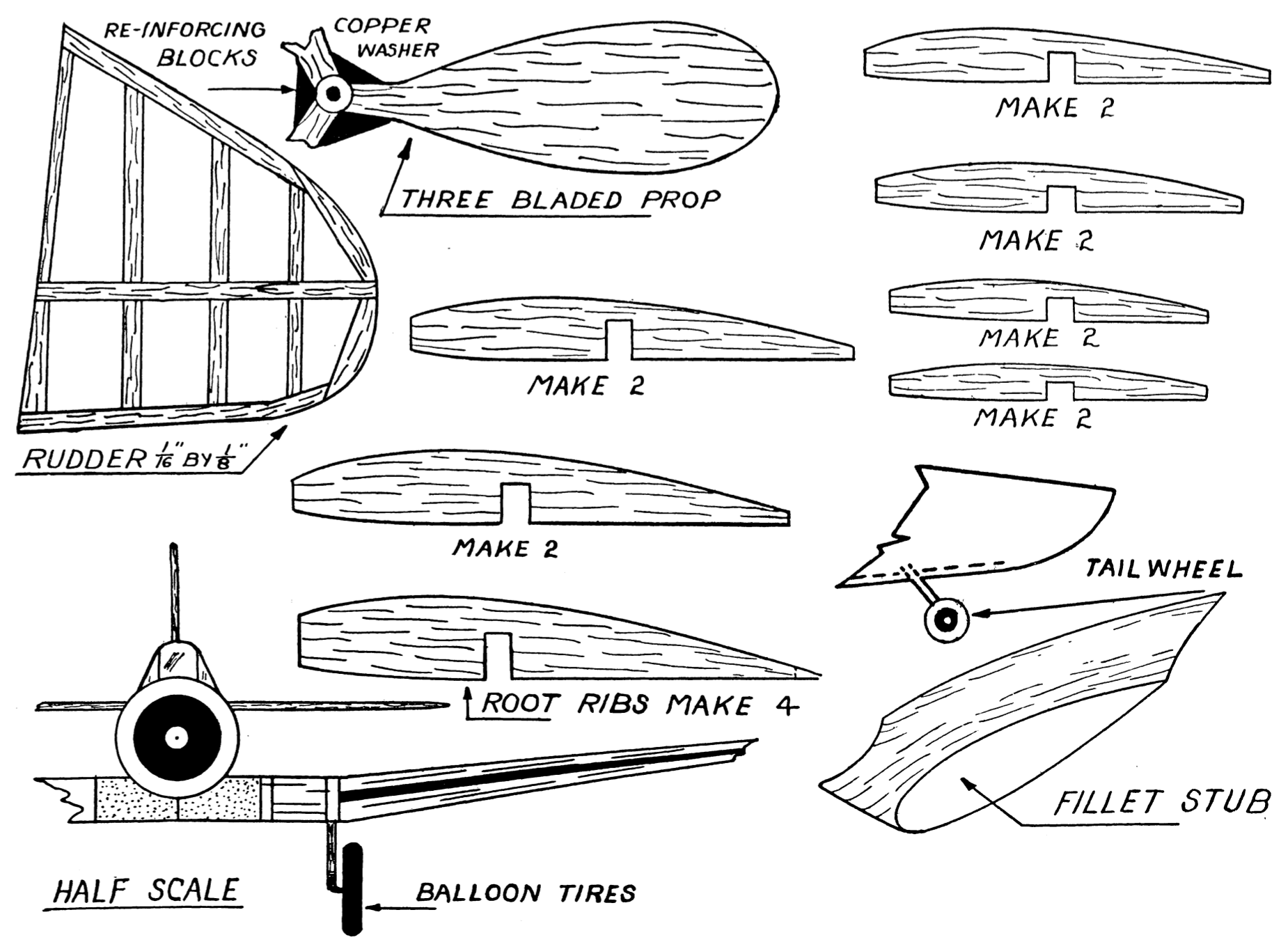
PLANS FOR THE DOUGLAS EXPORT-ATTACK FLYING ACES FEBRUARY, 1941
