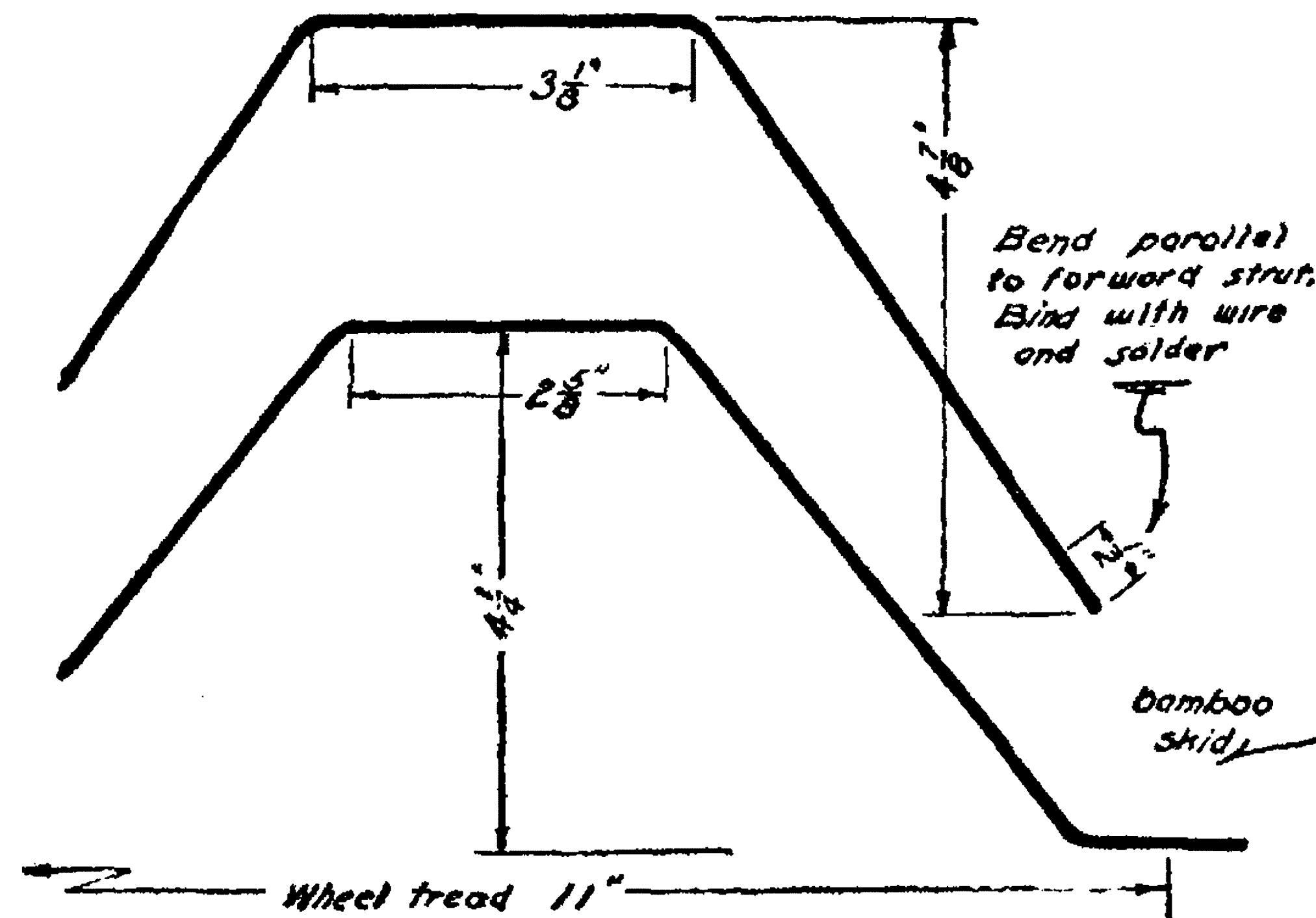
LANDING GEAR STRUTS 3/8" piano wire
