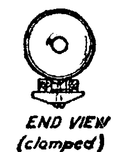
BATTERY MOUNT Cells are mounted separately; They are renewed by inserting new cells in the mounted jackets.
