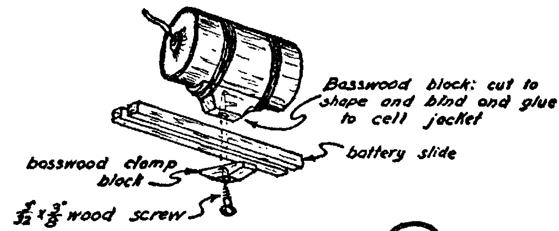
BATTERY MOUNT Cells are mounted separately; They are renewed by inserting new cells in the mounted jackets.
