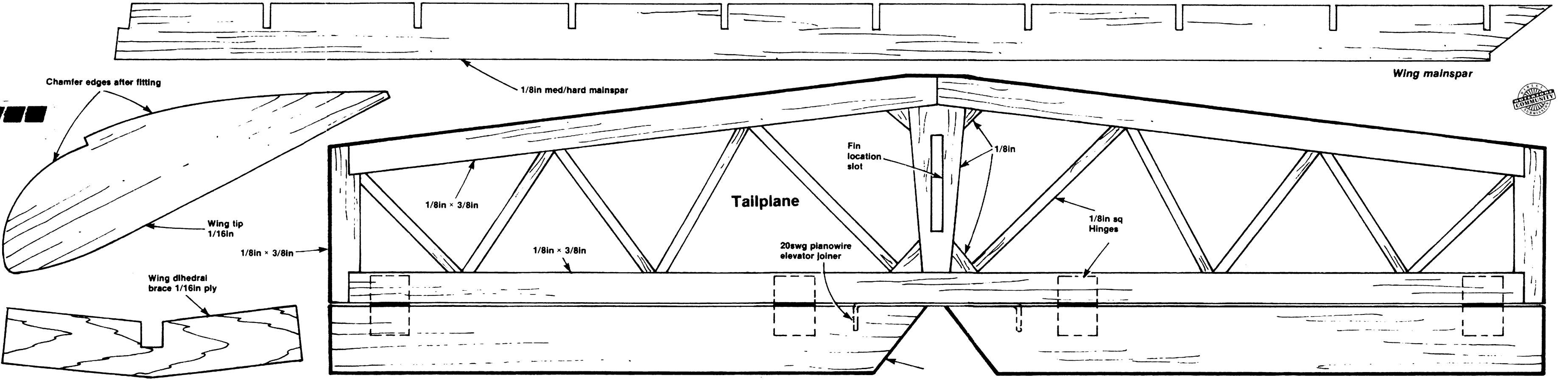
JIFFY 36inch span sports model for two function radio and .8 to 1.0cc engines Designed by Richard Preston
