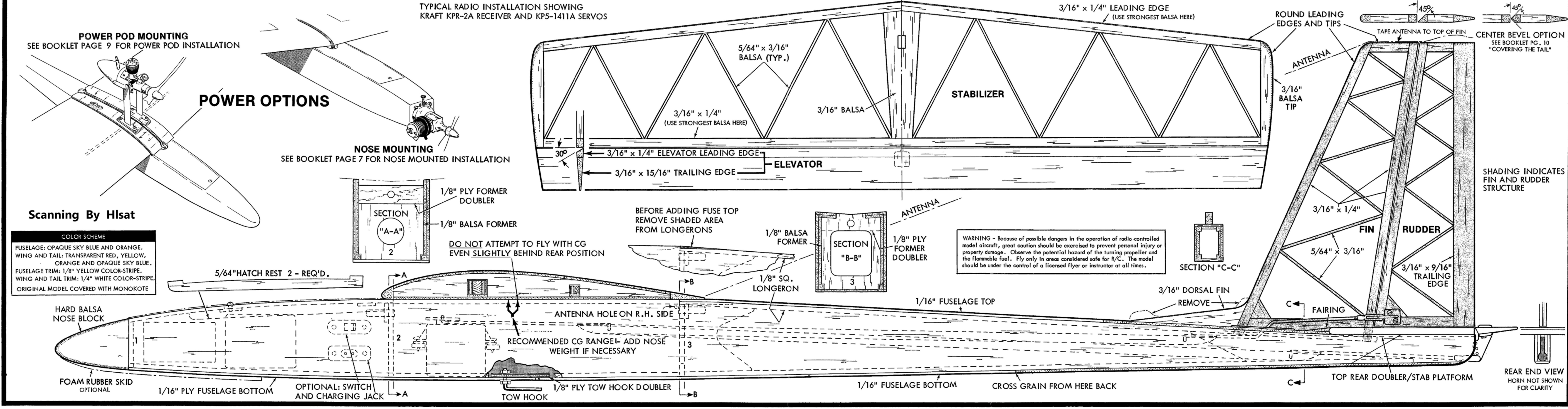
Gentle Lady - RC - Motor Glider - 78in.Wing - Eng .049 - .10 or Electric - from Carl Goldberg Models
