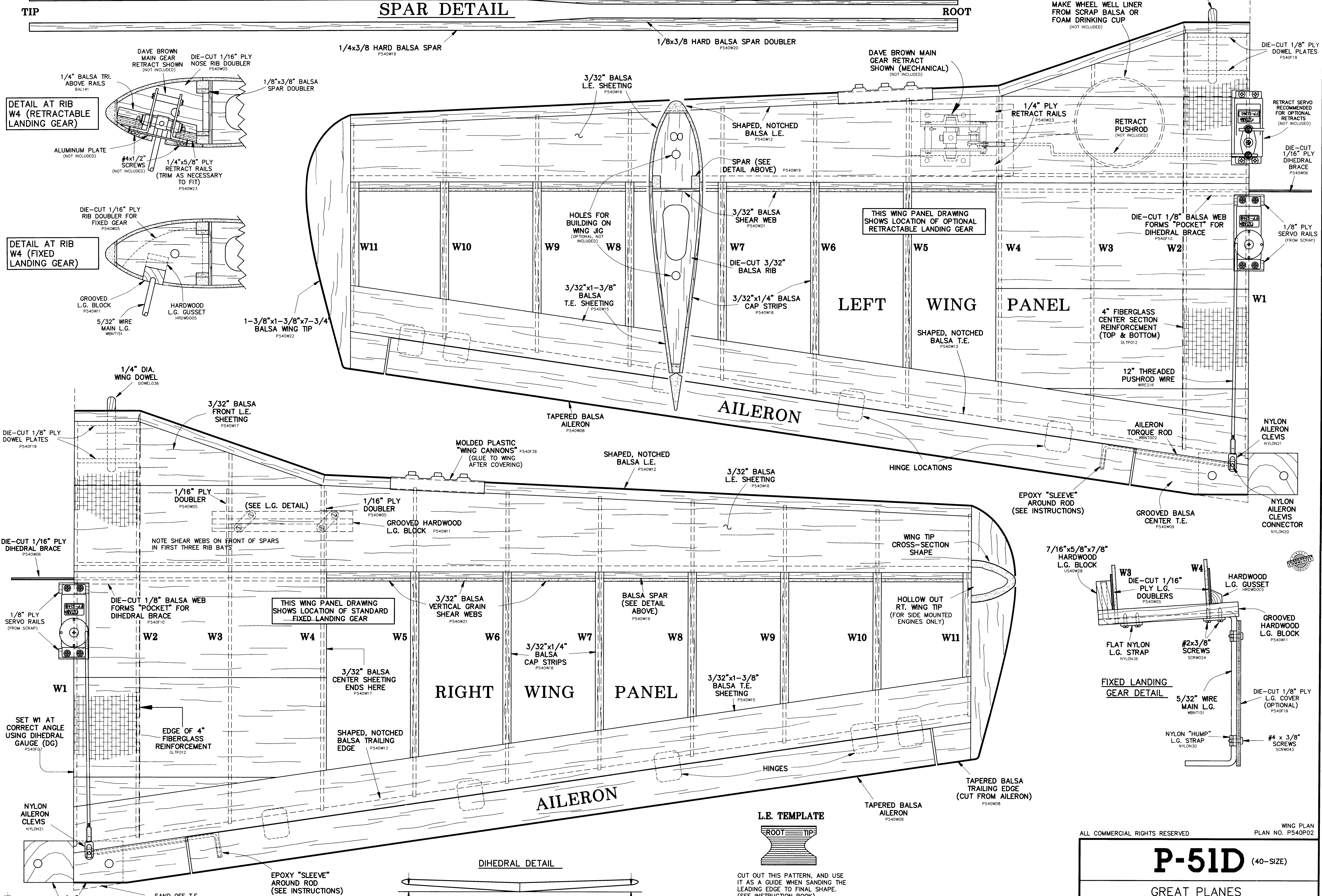
DIHEDRAL DETAIL
