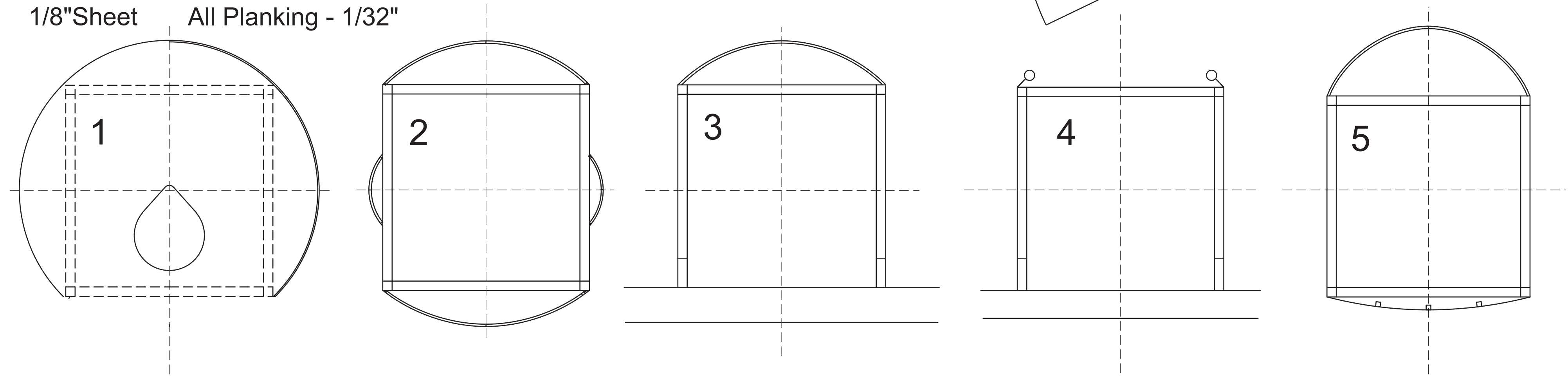
FUSELAGE CROSS SECTIONS - All Formers 1/16" Sheet Unless Specified
