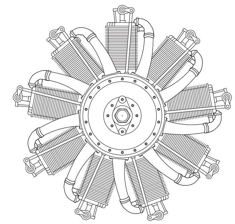
LeRhône Rotary 80hp
