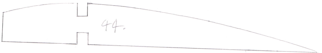
Capella Wing Ribs and Parts 36,37 Tracings
