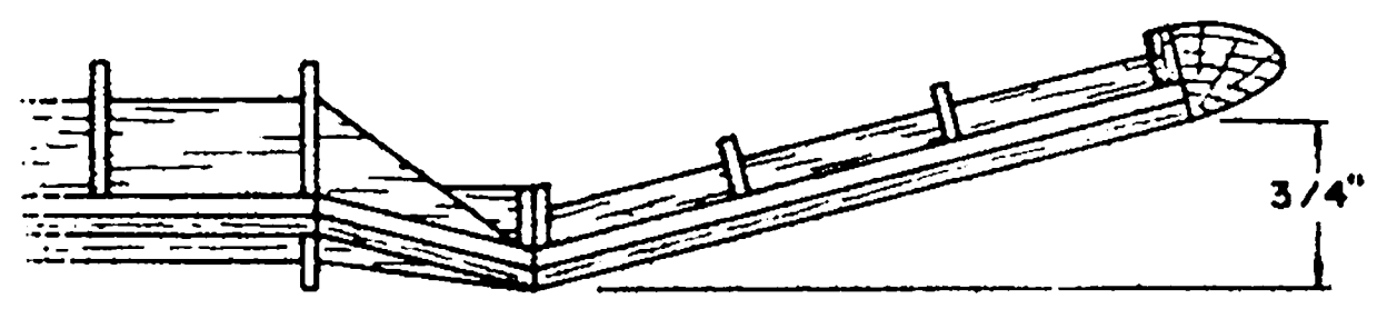
FRONT VIEW OF WING TIP
