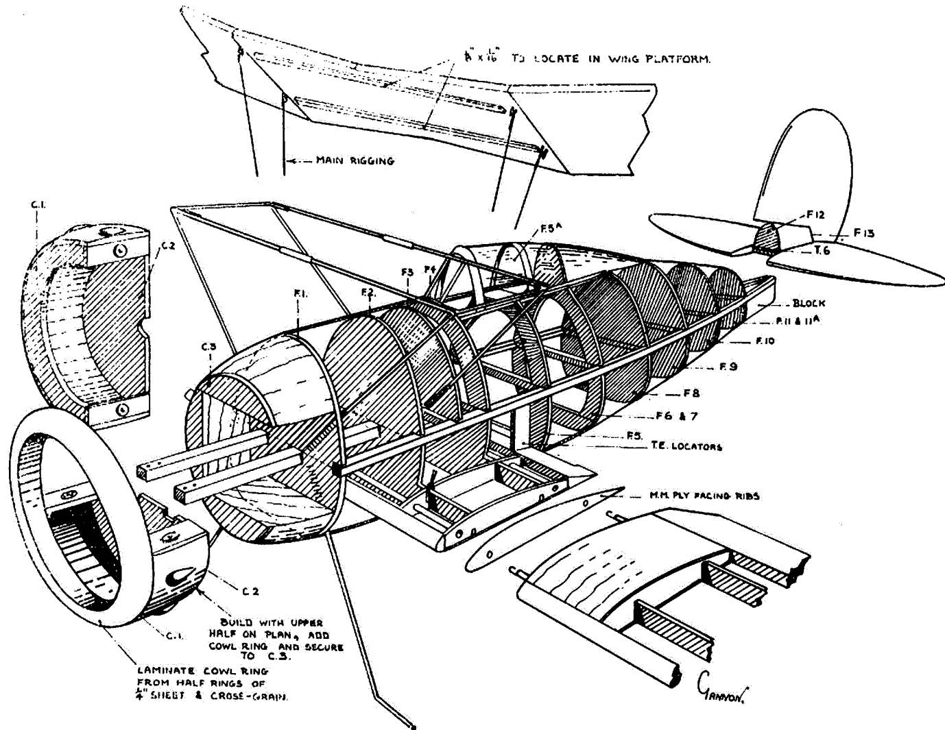
GLOSTER GLADIATOR ASSEMBLY DRAWING
