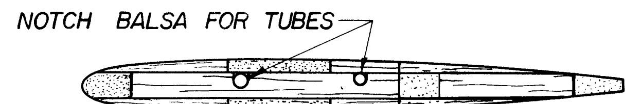
STAB SECTION AT ROOT
