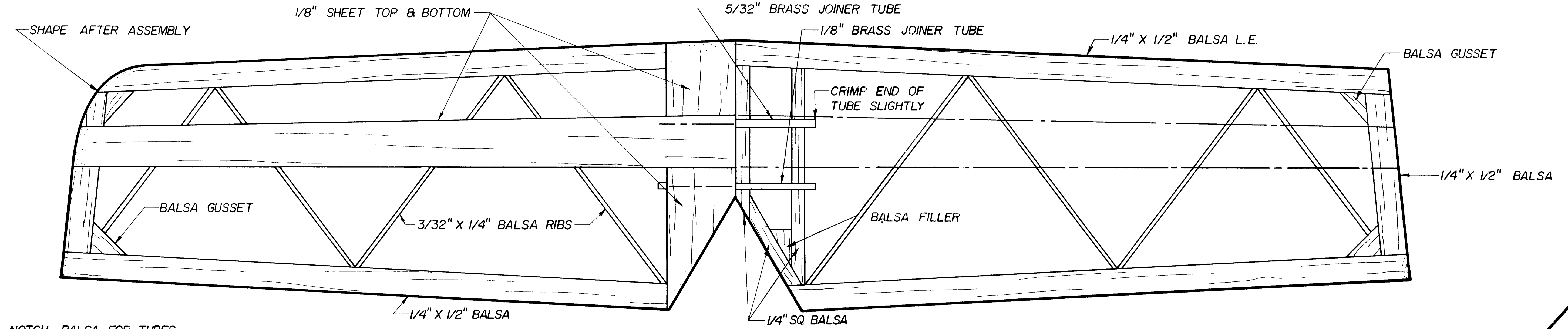
STAB SECTION (TYPICAL)
