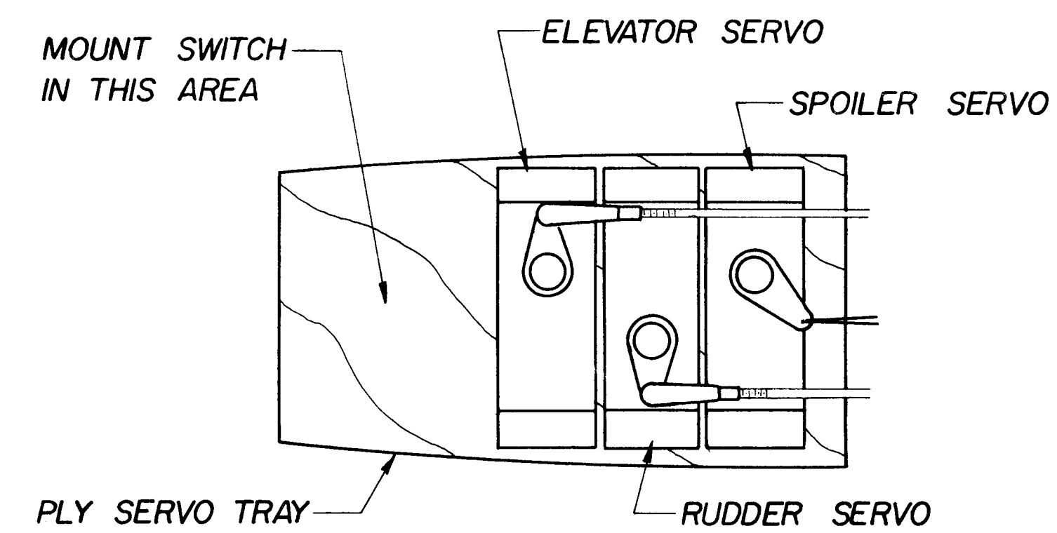
SERVO TRAY LAYOUT
