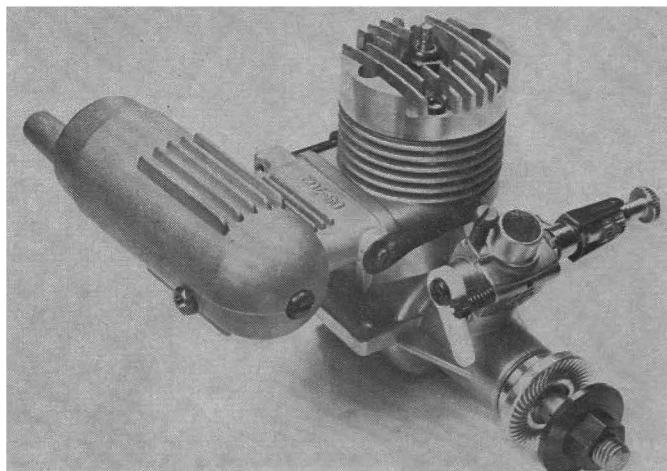
Current O.S. Max-25 R/C with type 21 carburettor. Good engine for the newcomer to R/C. As with all O.S. engines, an effective silencer is included with the Max-25 R/C.
