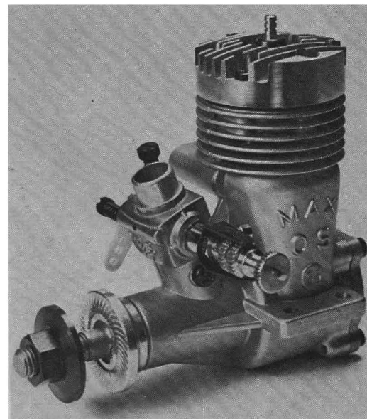
Current O.S. Max-25 R/C with type 21 carburettor. Good engine for the newcomer to R/C. As with all O.S. engines, an effective silencer is included with the Max-25 R/C.
