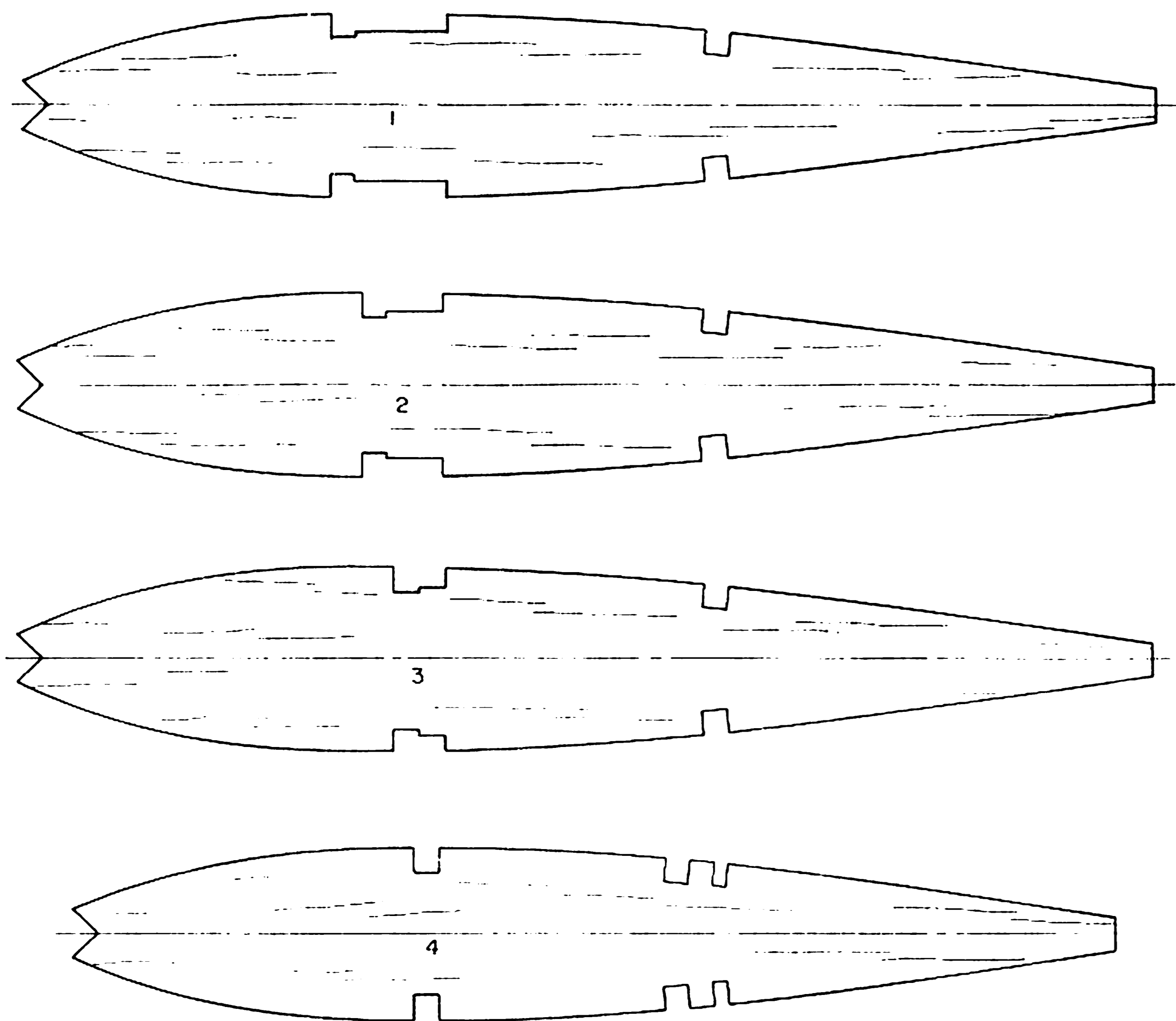
ALL RIBS CUT FROM 3/32" SHEET BALS
