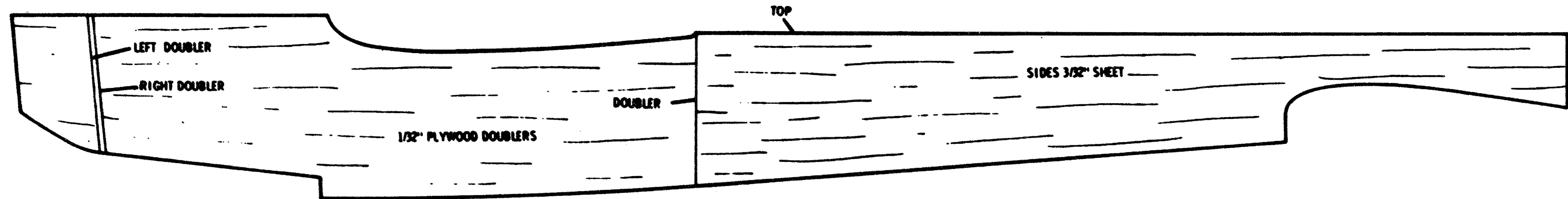
PATTERN FOR SIDES & DOUBLERS
