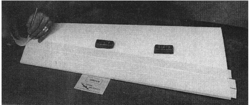
Apply wing sheeting tape to cores.
