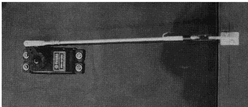
Futaba S130 installed, note 4-40 pushrod, soldered at servo end and Teflon tape wrapped at threaded end at elevon horn.
