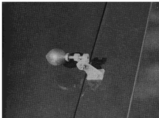
Method of elevon balance, 1/2 ounce sinker, link from elevon and cut down large control horn.
