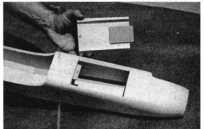
Hatch cut-out details.
