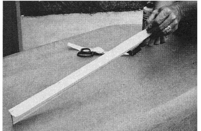
Pin X-hinge to center of leading edge of elevon.
