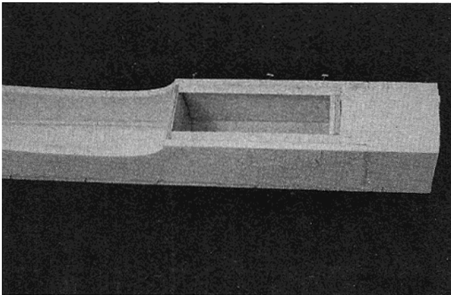
Left fuse side in place, nose blocked. Ready for bottom sheeting.
