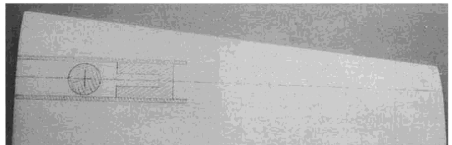
First step in building the wing, after cutting the foam cores, is to mark the locations of the stub spars, wheel, and landing gear plate.
