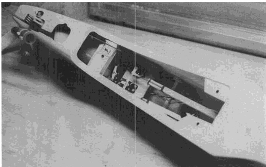
Radio installation. Note how everything is arranged in a clean and orderly manner. Also note the close-fitting cutout for the nose gear . . . nothing but first-class workmanship throughout!
