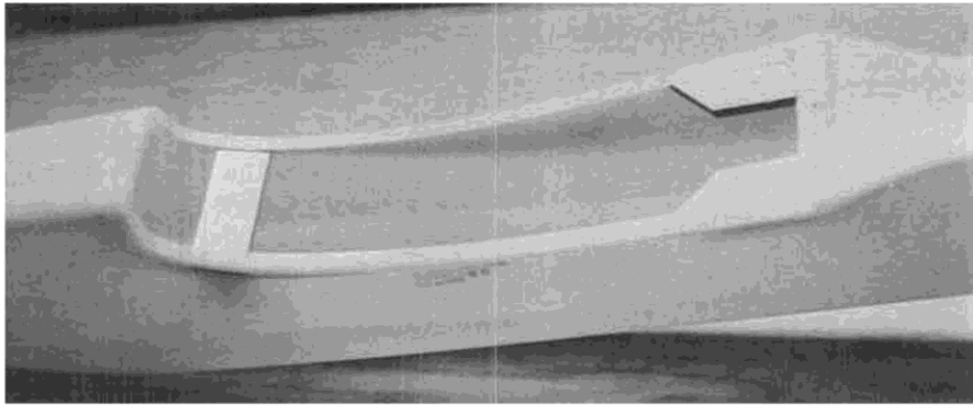
The plywood wing bolt mounts glued in place in the fiberglass fuselage.
