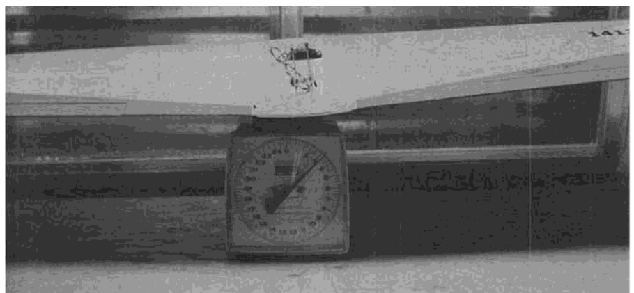
Completed wing, with servos and retracts installed, weighs 3-1/4 lbs. This is the maximum desired wing weight.
