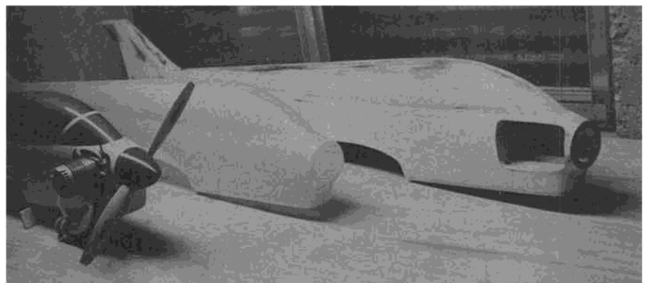
From l to r, a finished wooden fuselage, basic fiberglass fuse, and finished fiberglass fuselage. The fiberglass ones are available from W.K. Hobbies (see ad in this issue).
