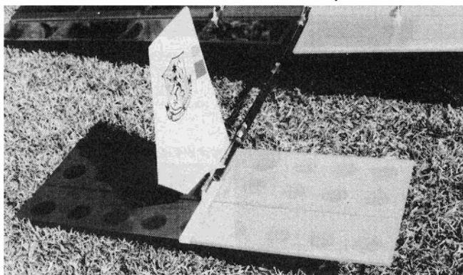
LEFT: Rear quarter view showing completed tail assembly. Also 1/16" M.W. pushrods and plastic guides taped to boom. RIGHT: Front quarter view showing tank taped to pod with foam rubber cushion.
