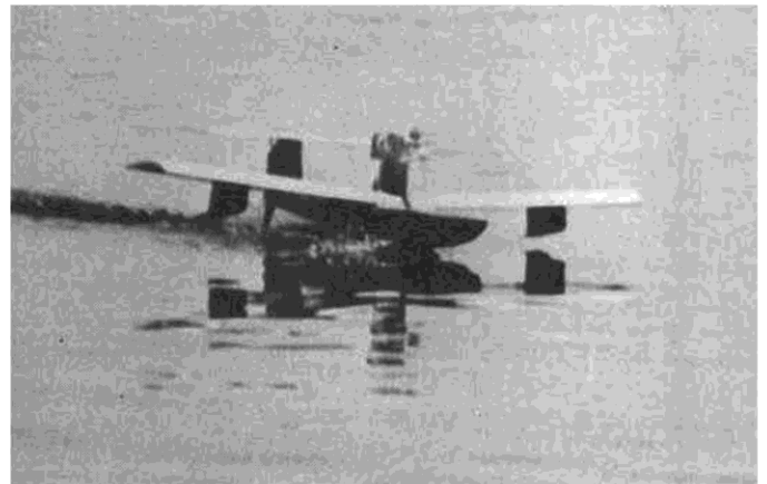
The wide bow keeps water out of the propeller path, thus avoiding loss of power during takeoff. Hull rides on planing skids at speed.
