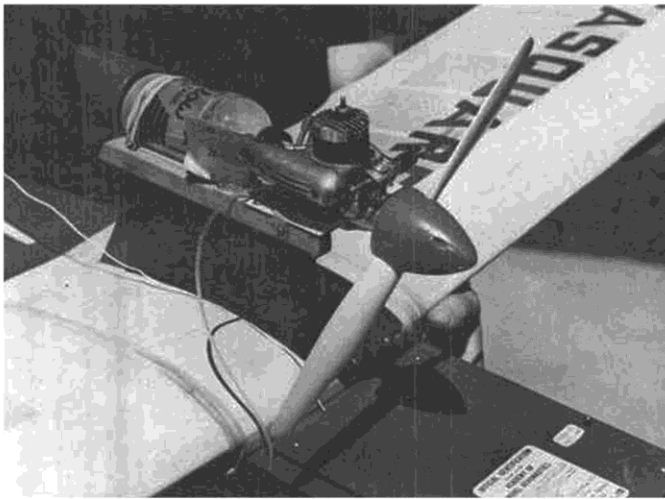
Engine pod is simple and open, makes things easy to get at. Note throttle control cable and exhaust deflector, also hatch cover.
