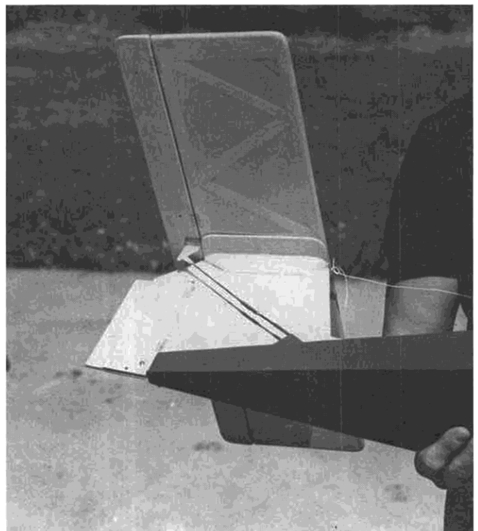
Control to the "T"-tail elevator may be exposed, but it sure is the easiest and most positive way to go. Sea rudder has been detached.
