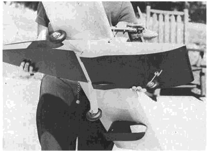
Underside photo shows demountable gear for land operation. Planing skids add a great deal to water handling at high speeds.
