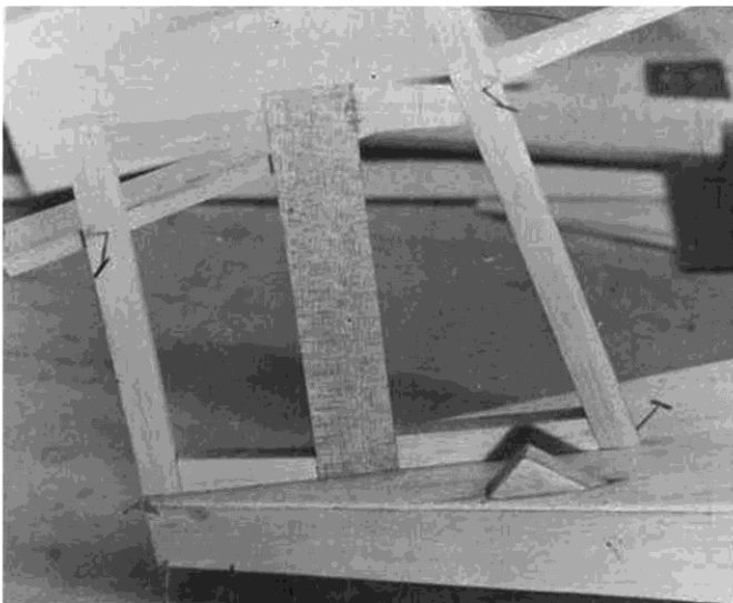
Fin, which supports the stabilizer on top, is sturdily built, and keys into aft end of the fuselage. Here, it is pinned to wood jig-piece.
