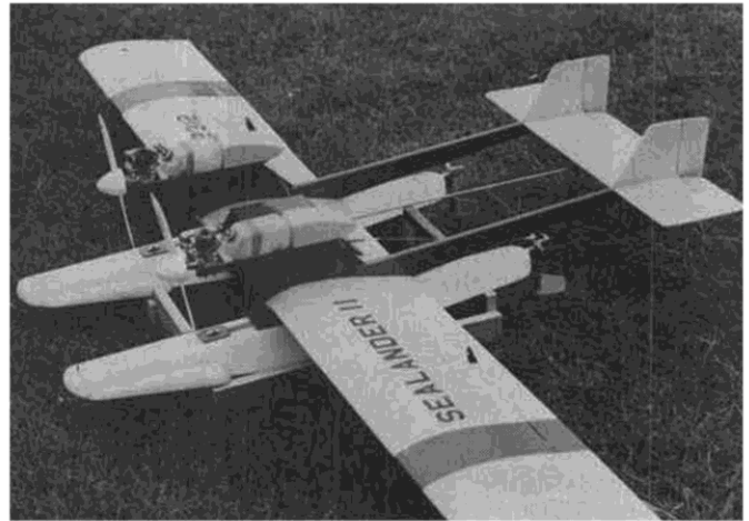
Both Sealanders have sponsons added to the floats. Lowers waterline and also deflects water spray away from props.
