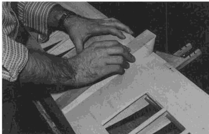
John Ross illustrates how to sand curvature on bottom of float mount. Put sandpaper face up on wing, move mount sparwise.
