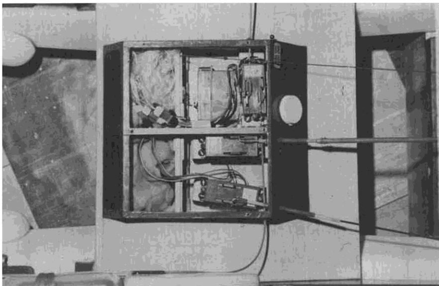
R/C equipment installation in Sealander II. Cover is gasketed to keep out water. Servos, linkages, and other gear easily accessible. Pill bottle top idea by Lenny Poor. Really works well.
