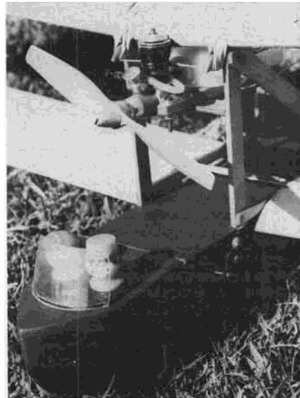
Tank straps to engine rails. Rails may be extended aft for tandem twin power, if you want some wild action.
