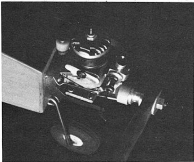
Kink in throttle pushrod provides override protection for servo. Note small gauge wire used. Adjustment is at servo end.
