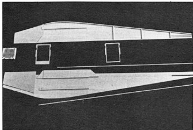
First step in fuselage assembly. Be sure you make a left and a right! Cabin doublers notched to fit over ply nose doubler.
