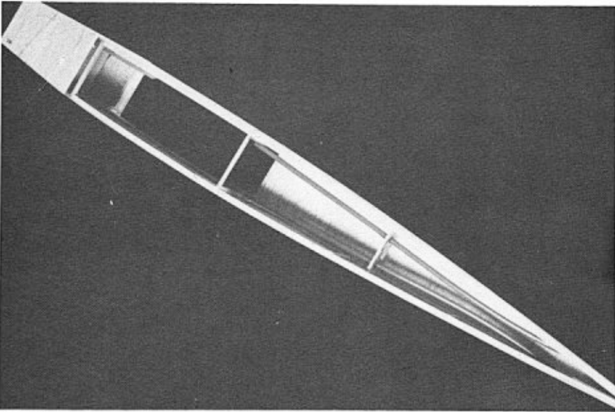
(Top) Sides are joined, ready for installation of the firewall. (Btm) Bottom has been sheathed, crossgrain, and tail surface control Nyrods installed.
