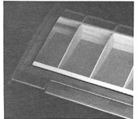
Wingtip close-up shows tip plate and anti-stall tab. Trailing edge piece is simply reversed.
