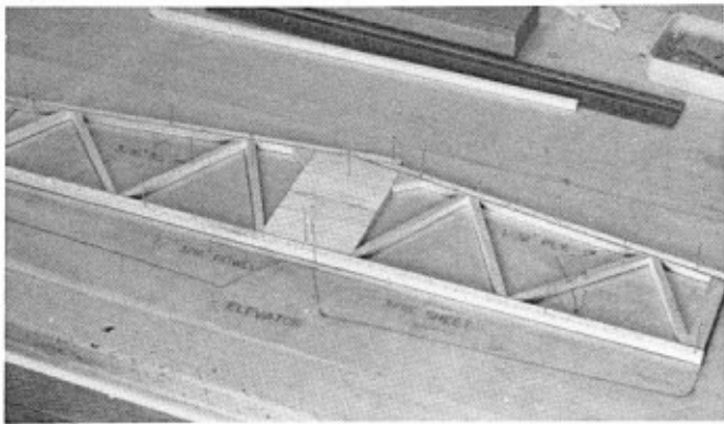
Stab framework pinned down for drying. Note the 1/32 ply leading edge doubler. Also used on main spar.
