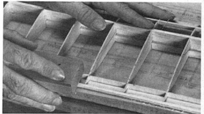
Sanding block is used to prepare structure for trailing edge sheeting.
