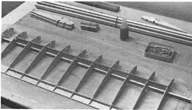
Accurately cut, vertical grain, spar webbs are an aid in obtaining correct rib alignment. Make yourself a "kit" before assembly starts.
