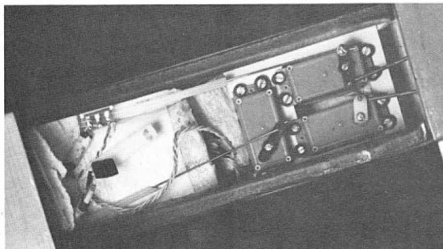
Radio installation, nose to left. Servos are mounted on plywood tray which is epoxied to side rails in fuselage.
