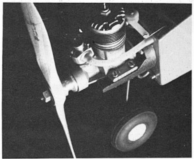
Nose gear steering linkage and fuel line installation shown in this photo. Set-up is simple and trouble-free.
