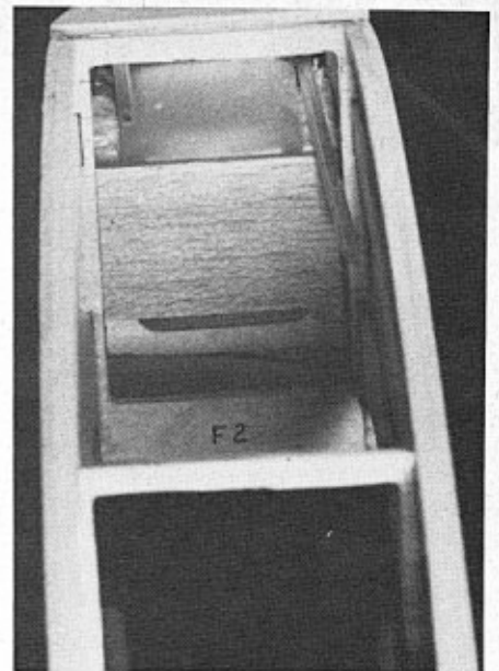
Looking toward the nose, showing tank and Nyrod installation.
