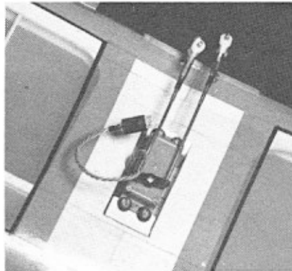
Aileron servo installation details.
