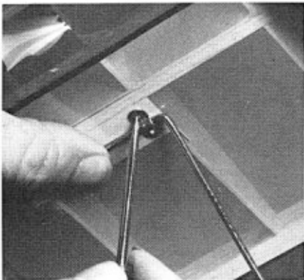
Main landing gear struts retained with metal brackets. No time for screwdriver to slip!
