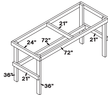
WORKBENCH FRAME
