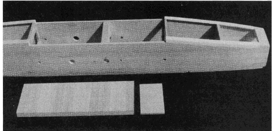
Bottom of fuselage ready for main L.G. plate and radio compartment hatch. Note cross grain sheeting on hatch.
