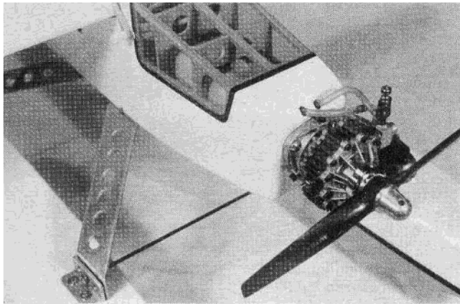
O.S. Wankle comes with aluminum radial mount. 1½° aluminum wedge gives needed right thrust. Note music wire spreader and soldered nut keeps on float gear.
