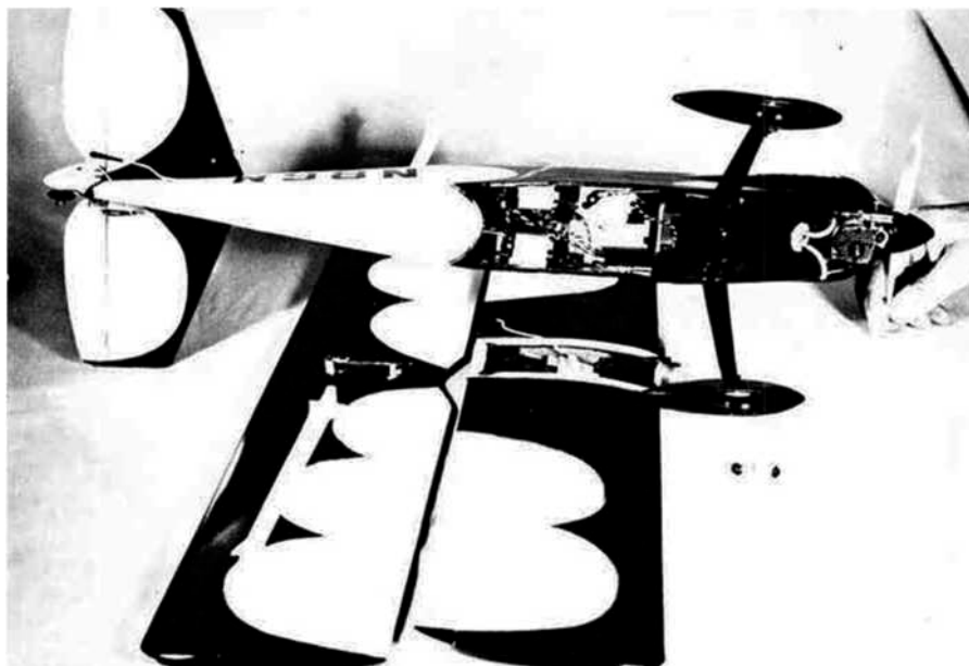
The Mongster's radio installation makes use of coupled rudder and ailerons. Note coupling link attached to aileron bellcrank. Arrangement saves space and weight. Wing struts plug in.
