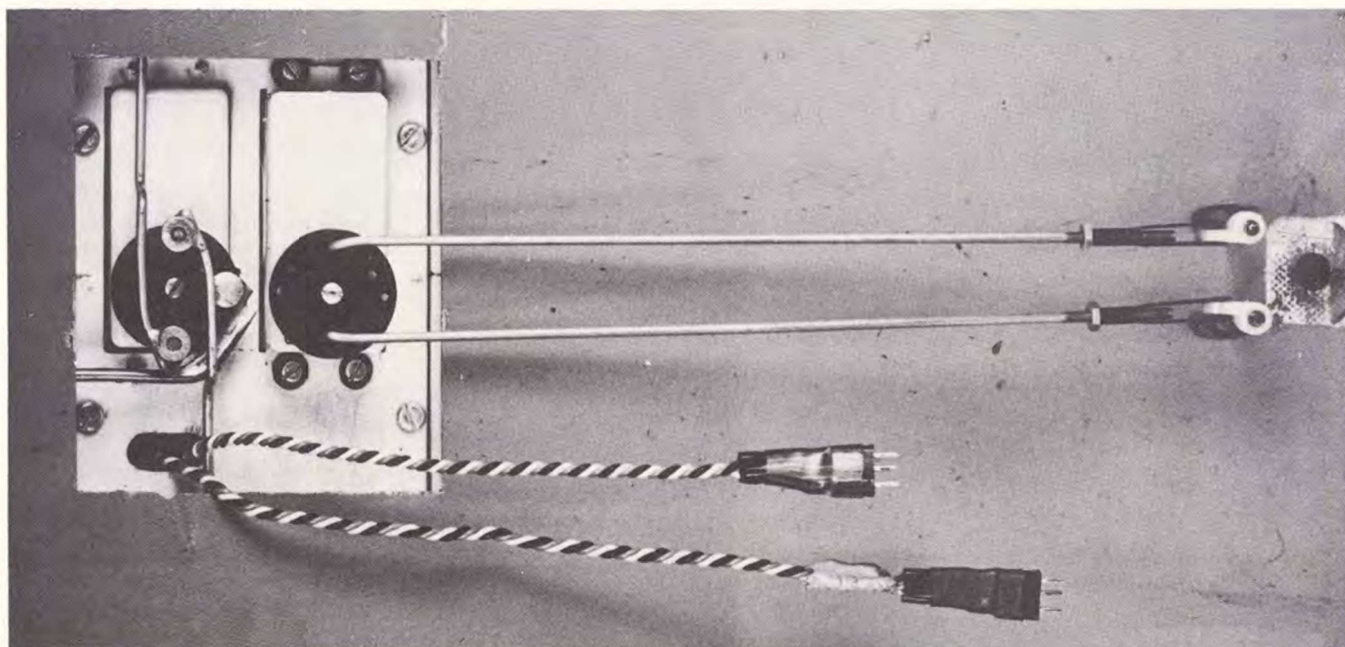
Close-up of aileron and retract servos—Z bend used for aileron pushrods,
