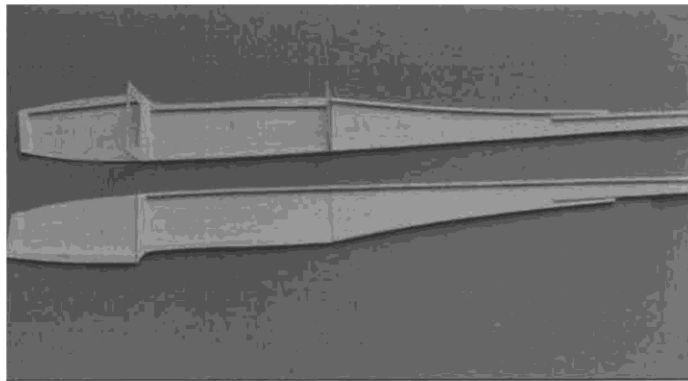
Fuselage sides ready for joining. The right side is cut 1/16-inch short at the nose to produce needed right thrust when the motor is mounted.
