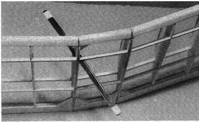
These two pictures, (above and below), show the method used to cut the slots for the plywood gussets. Two hacksaw blades are tapped together to achieve the desired thickness of cut. Plans clarify.
