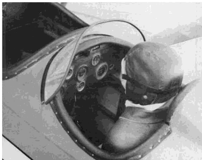
Not many, but enough! Instrument panel in G.L.T. was sparse but adequate. Note on-off switch that caused radio problems.
