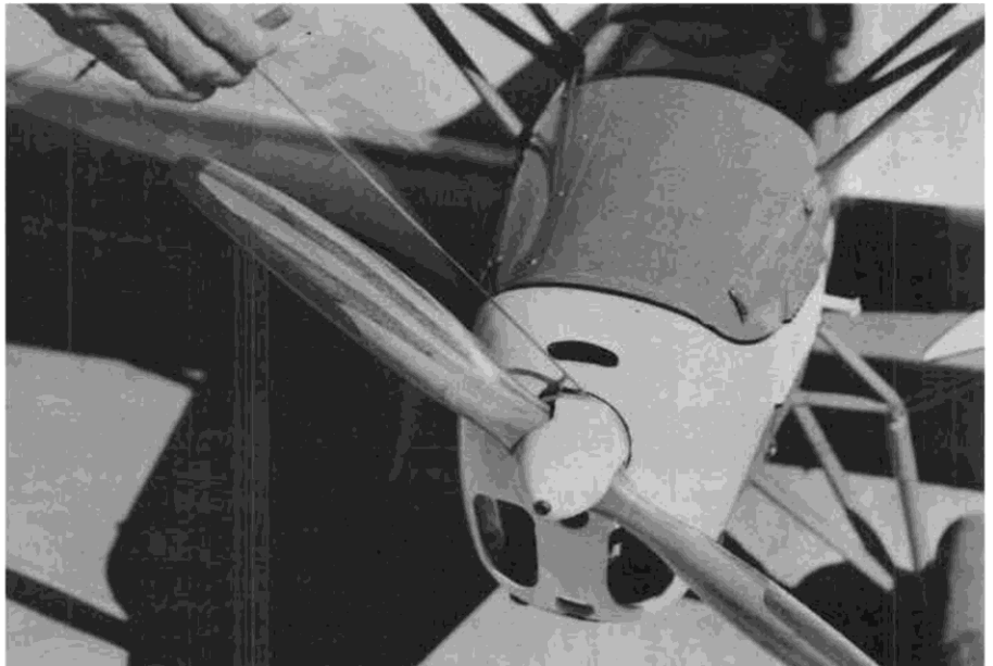
Close-up of cord starter, ready to spin prop. A 30-inch cord with knot in end is just right for the job. Note fingers are clear of prop blades.
