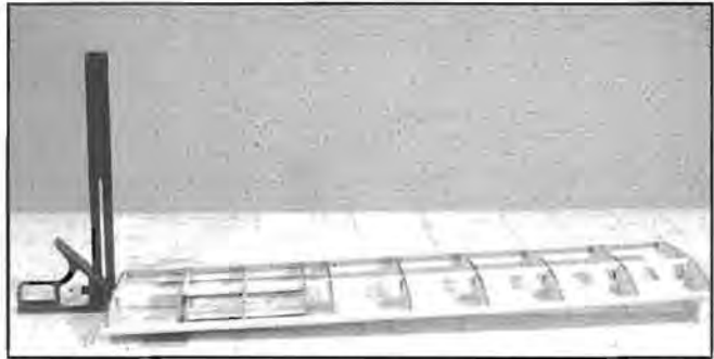
LEFT: Trim the lower sheet with an X-Acto knife and straightedge. RIGHT: Setting the root rib at the correct angle using a square and a 1-1/8" block.
