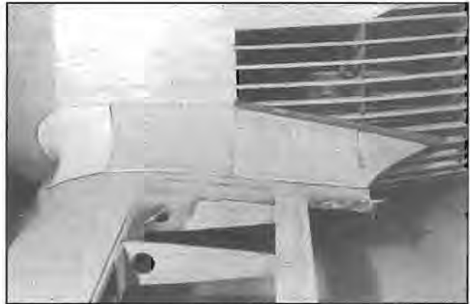
LEFT: If you glue WF4 to the plastic fillet front, you won't have to measure anything to get in the right place on the wing. Be sure to glue it only halfway across WF4 to leave a flange for the 1/16" sheeting. RIGHT: The fillet is sheeted with 1/16" balsa. The fillets were hammered out of aluminum by hand on the full-scale plane so you don't need to be too fussy here.
