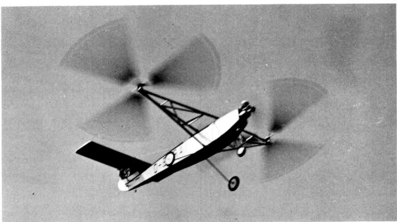
The FA 61 makes a slow pass overhead for the photographer. With full back stick, the ship will mush along at about 10 mph. Ship will even fly when out of trim, but looks strange.
