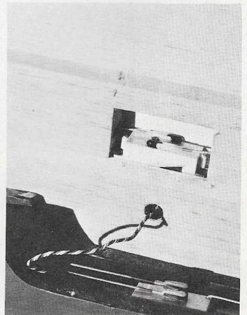
The modular wing center section houses the spoiler servo. The model disassembles very quickly and stores easily with this arrangement.
