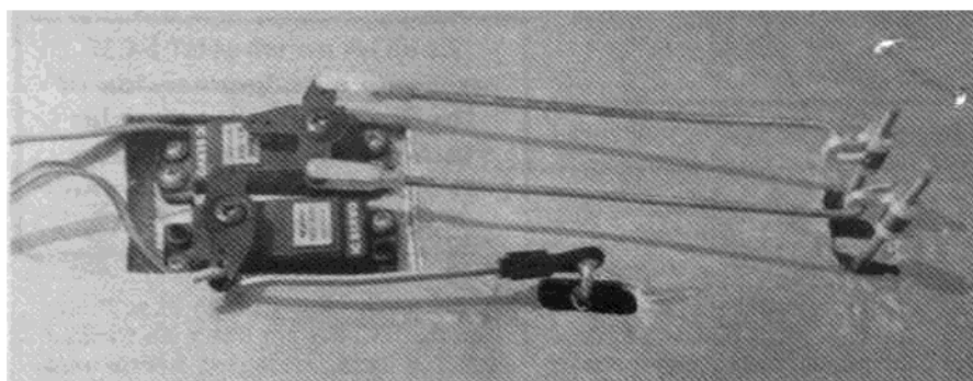
Aileron and throttle servos mounted in wing. Both operate torque rods with the throttle having pushrods at outer ends of torque rod.
