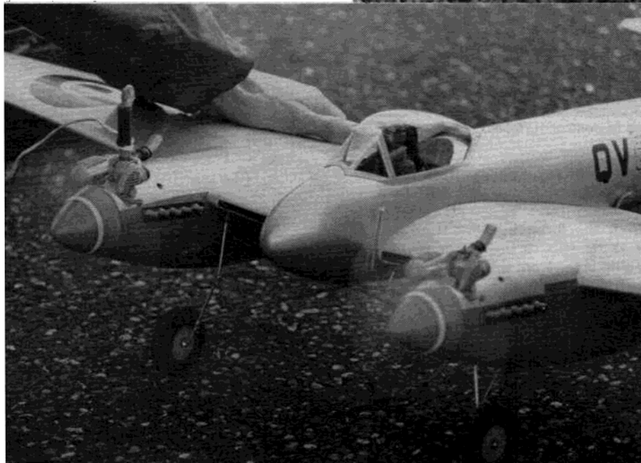
ABOVE: Prototype with O.S. .10s installed. Note muffler extensions to blow exhaust away from wing. LEFT: Hornet rests on its dolly. This is used when a smooth runway is available.
