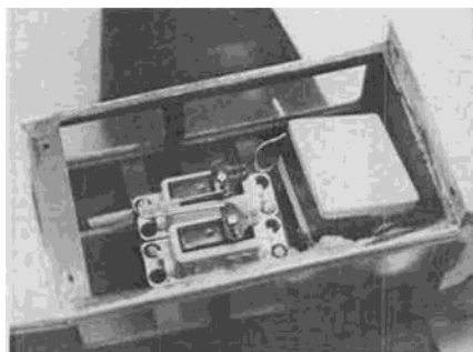
The front end of the Gold-N-Rod shows the working side of the three element system. Use some Super 'T' to secure elevator rod.
