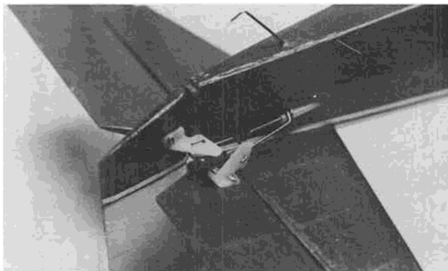
This Airsedan uses a three element push rod system based on the old stand-by, the Gold-N-Rod. The outer nylon rod is securely fastened to the fuselage, the inner rod has a friction tight wire wrapped around it, and there is another wire inside for rudder.
