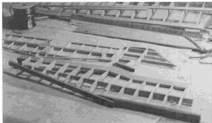
The author prefers not to cut individual tip ribs for the lower half-wing, so instead, he makes them the correct length, depth, and with the correct spar notches, then, using the root ribs as templates, simply sands in the airfoil shape. Simple, effective.
