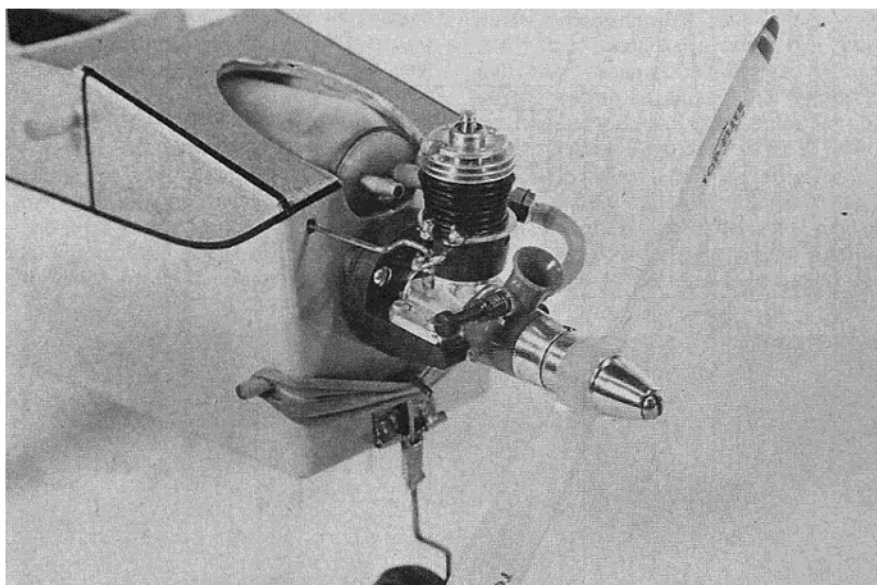
Close-up of motor mount, throttle linkage.
