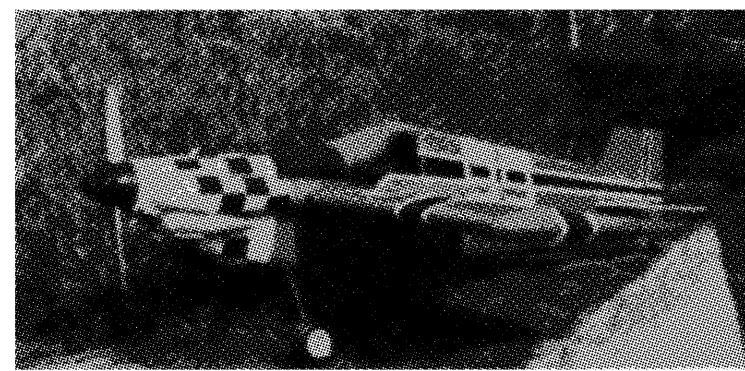
Side view of the "Cassutt" shows how that O.S. Silencer nestles neatly below the dummy cylinder side cheek cowling.
