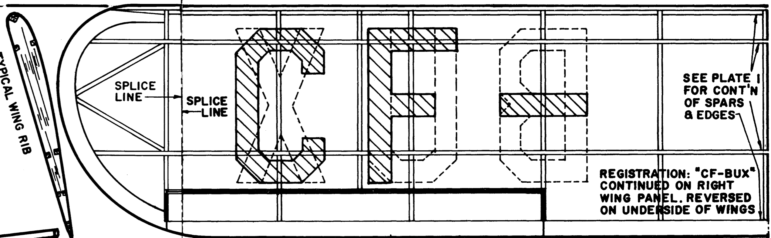
MAKE ONE WING & ONE SET OF STRUTS AS SHOWN & ONE OPPOSITE-TWO TOP WING SPARS TO RUN IN ONE PIECE FROM TIP TO TIP PIPER "CUB" J-3 PLATE 2 of 3 N.Charlebois
