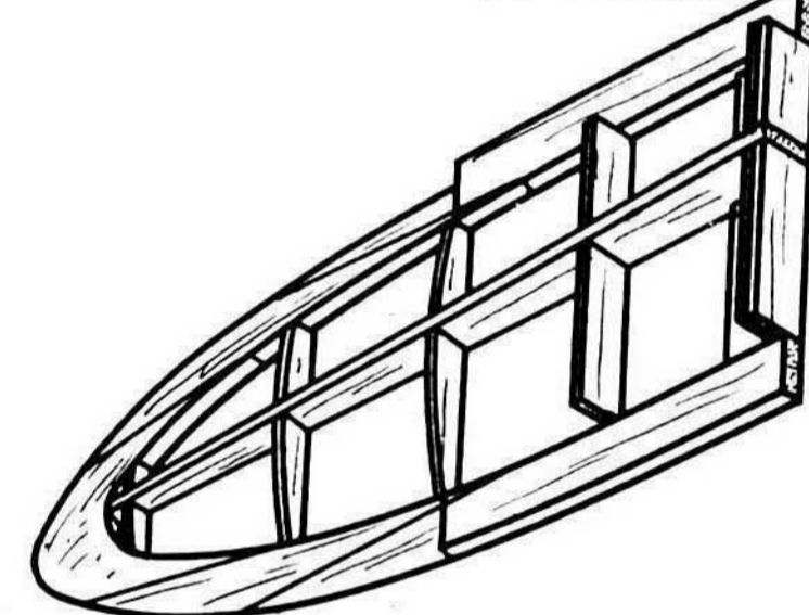
STAB LAYOUT
