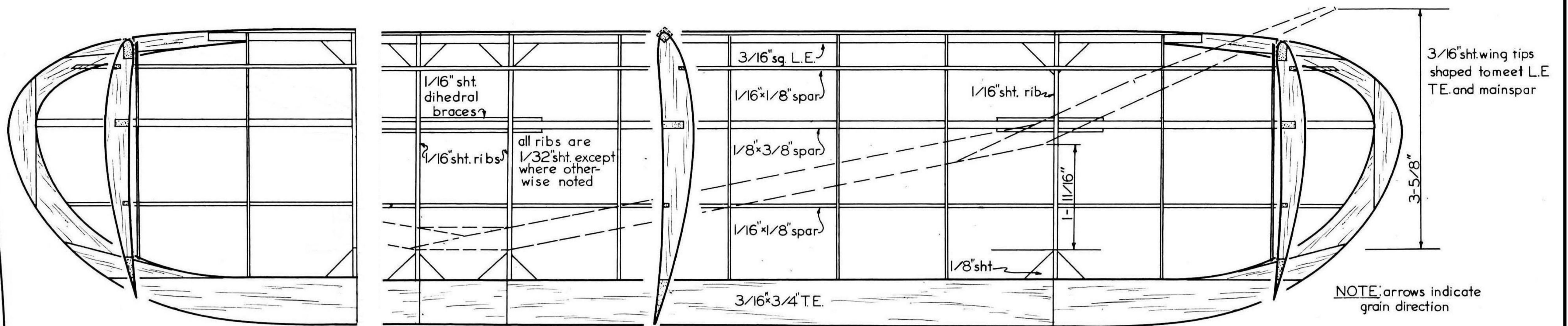
STAB LAYOUT
