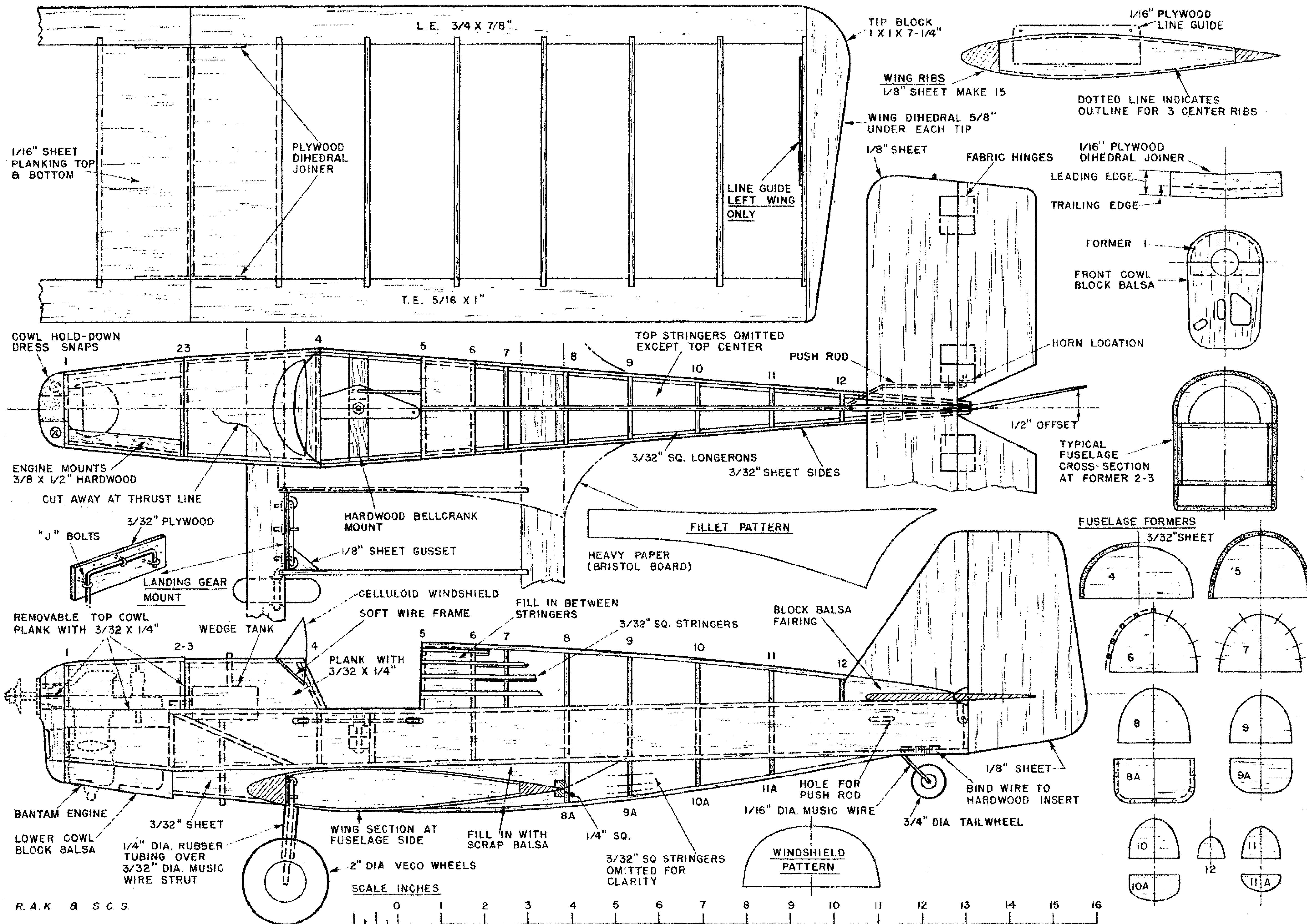
• Actual size working drawings for building Topsy are part of Air Trails Full-Size Plan #1049!
