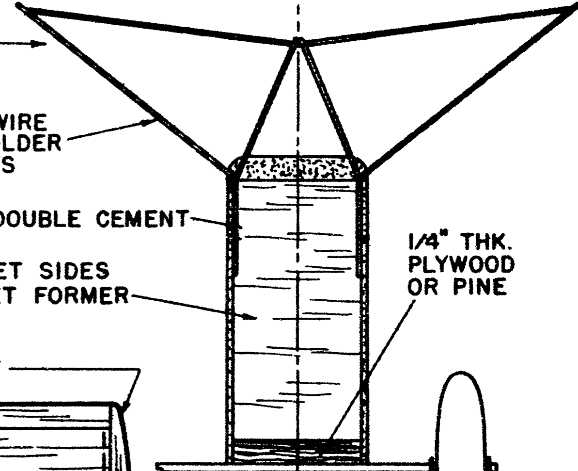
SECTION AT FRONT OF WING MOUNT
