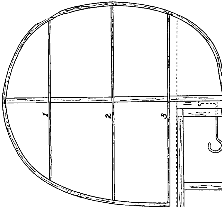
RUDDER RIBS
