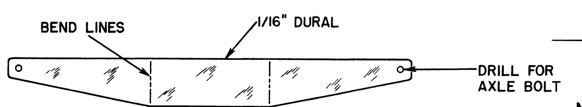
LANDING GEAR LAYOUT
