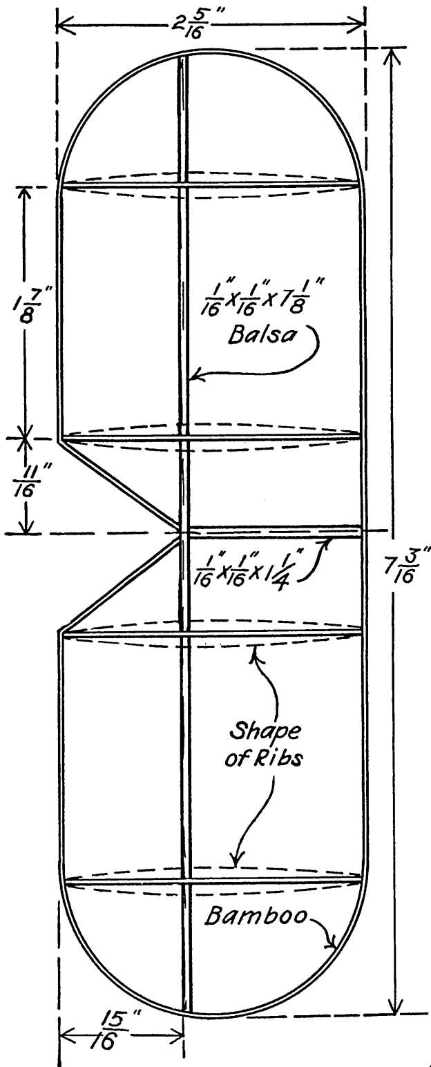
ELEVATOR
