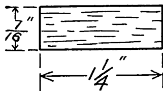
PONTOON BULKHEAD 8 No. 5
