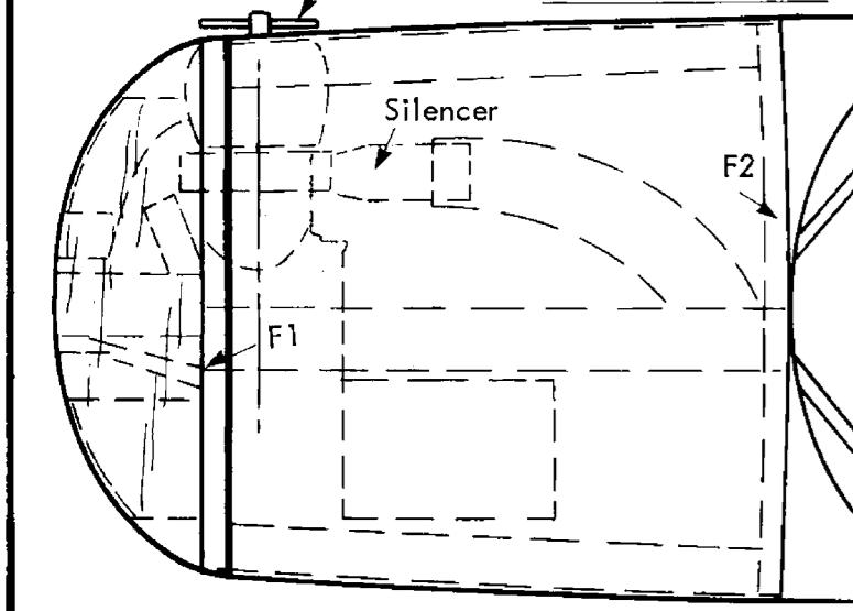
Albon "Dart" 0.5cc diesel shown SMALL SCALE FRONT VIEW OF FUSELAGE
