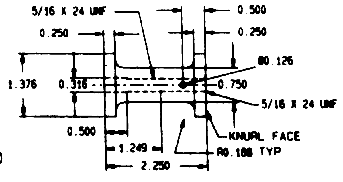
PROP EXTENSION DETAIL
