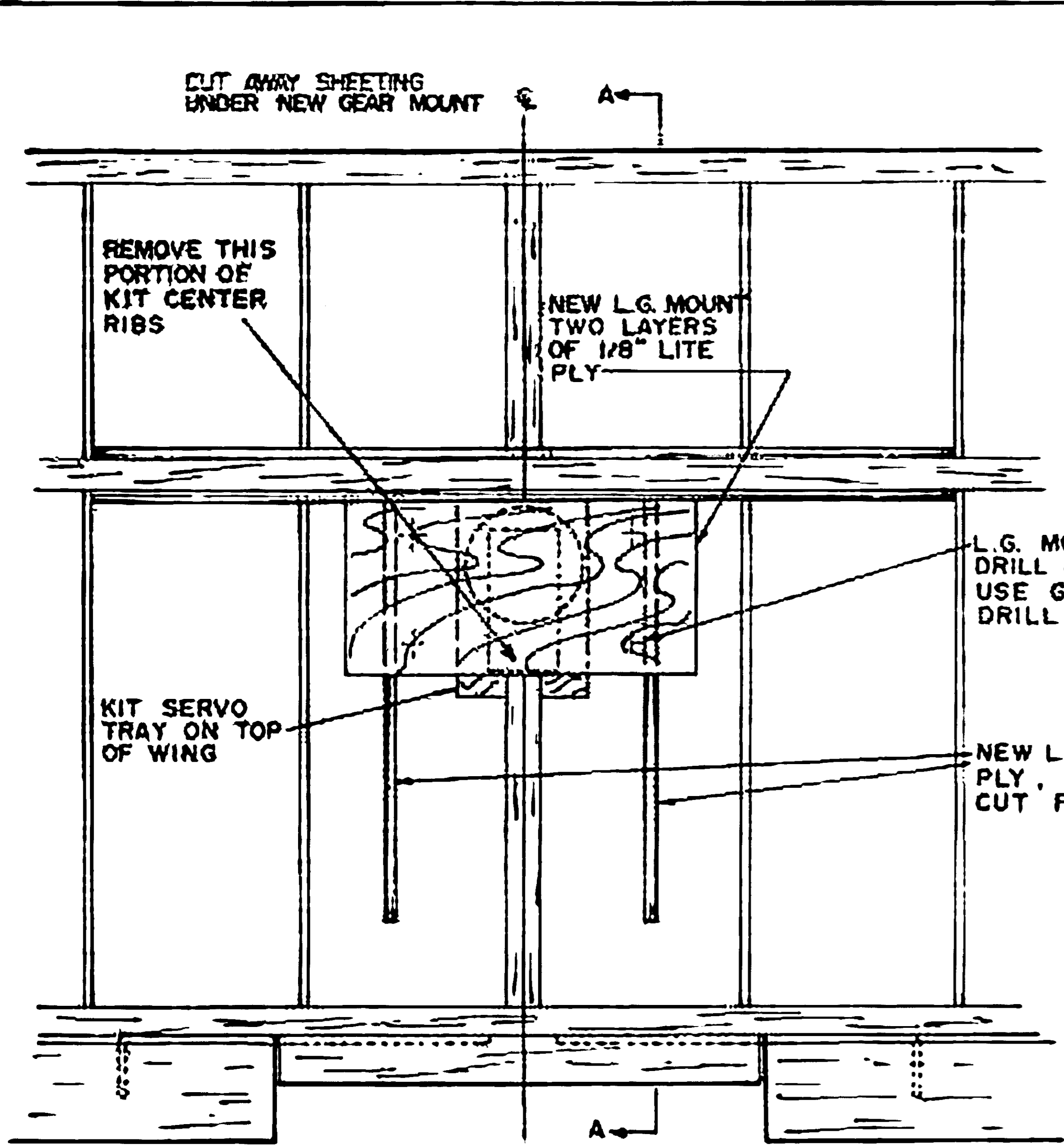
WING BOTTOM VIEW (SHEETING OMITTED FOR CLARITY)
