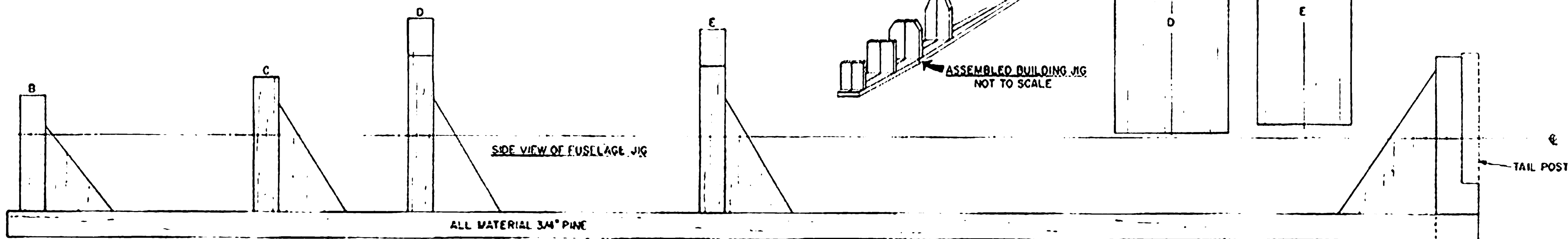
PLY FUSELAGE BUILDING JIG
