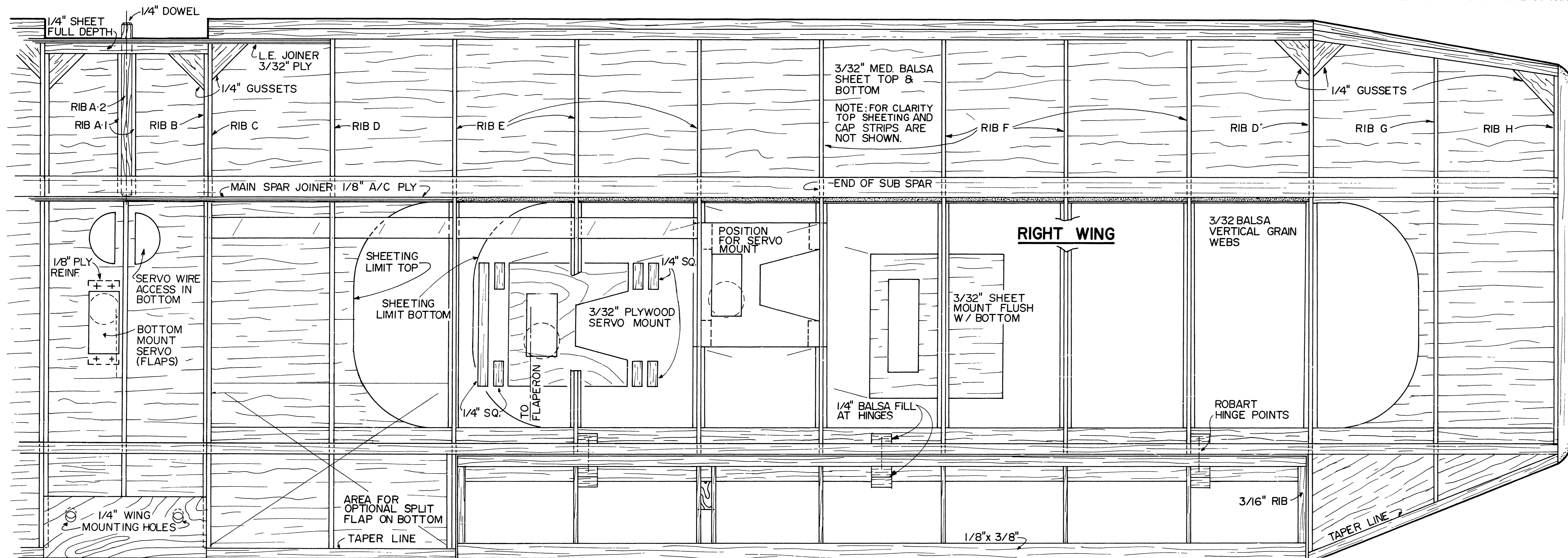
COMPOSITE VIEW OF MAJOR WING STRUCTURAL ELEMENTS
