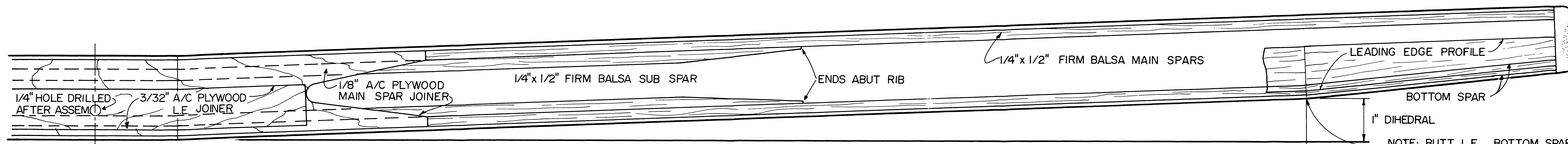
COMPOSITE VIEW OF MAJOR WING STRUCTURAL ELEMENTS
