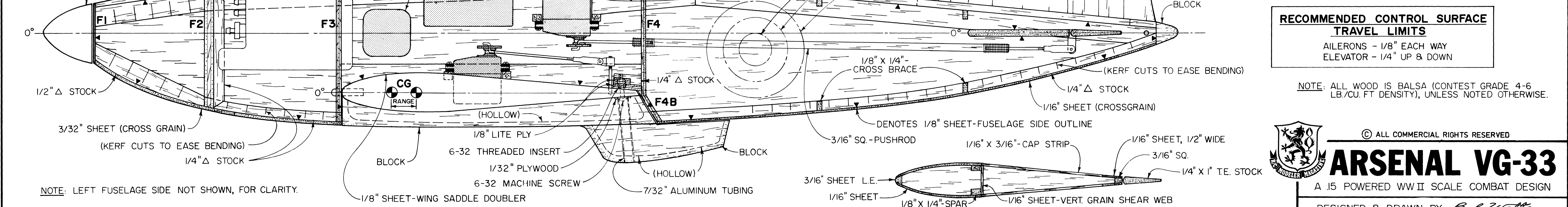
TYPICAL WING SECTION
